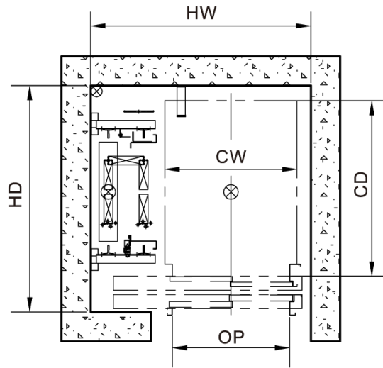
HOISTWAY PLAN OTHER FLOOR
