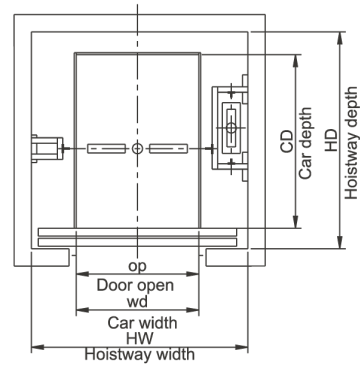
HOISTWAY PLAN
