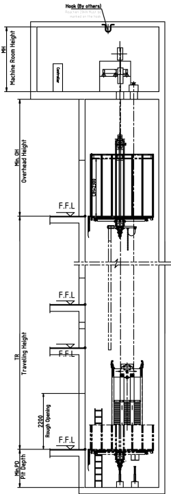
LIFT SHAFT - SECTION VIEW
