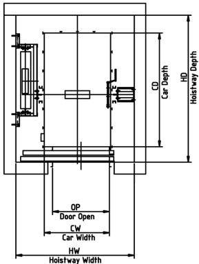
HOISTWAY PLAN
