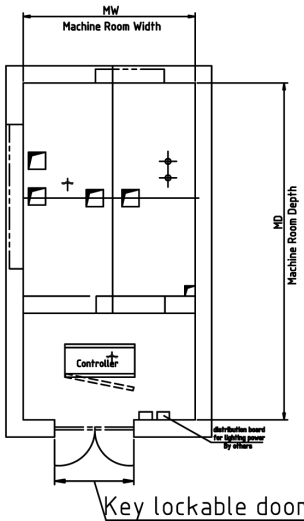
MACHINE ROOM PLAN
