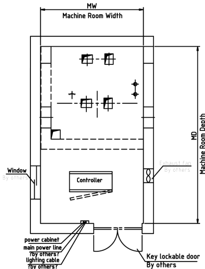
MACHINE ROOM PLAN
