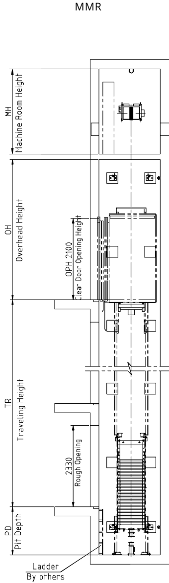
LIFT SHAFT - SECTION VIEW
