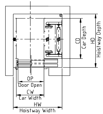
HOISTWAY PLAN
