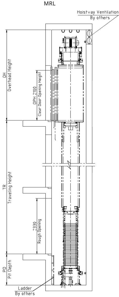
LIFT SHAFT - SECTION VIEW
