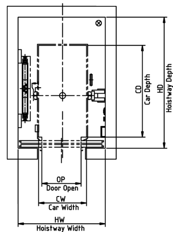
HOISTWAY PLAN
