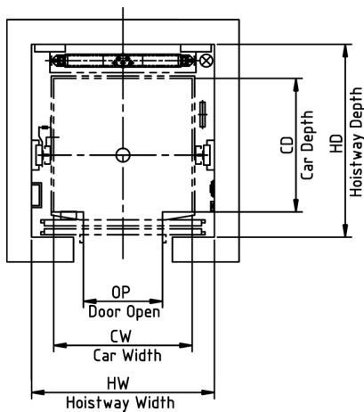
HOISTWAY PLAN
