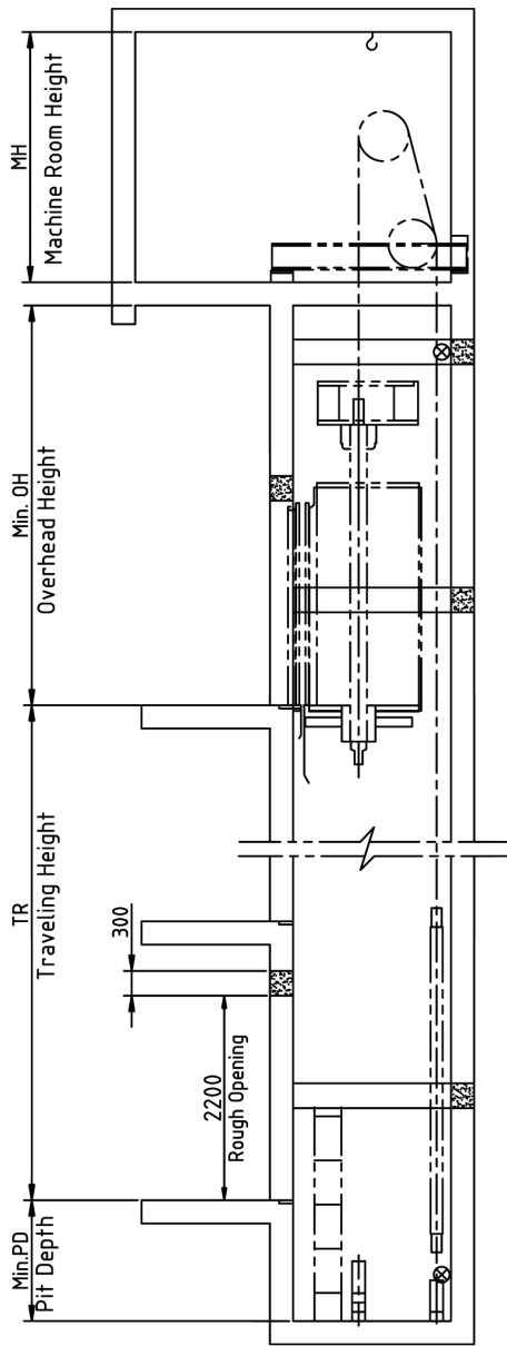
LIFT SHAFT - SECTION VIEW
